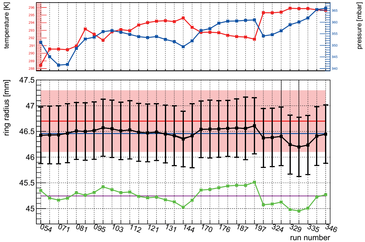
Figure 5.9. – Bottom: Mean ring radius for Position A for 33 different runs (black) covering a time period of roughly 12 days. The error bars mark the widths of the radius distribution (Gaussian shaped) of each run. In blue the mean value of all 33 ring radius distribution-means from these runs is shown ( \approx 46.46 \text{ mm} \pm 0.02 \text{ mm}_{\text{RMS}} ), and in red the mean value and distribution width from simulations ( r_{\text{mean, sim}} \approx 46.7 \text{ mm} , \sigma_{r, \text{mean, sim}} \approx 0.6 \text{ mm} ). Additionally in green the uncorrected values from the runs are plotted with the mean of the uncorrected data in purple. For readability only every second run number is given. Top: Corresponding temperatures (red) and pressures (blue) inside the RICH prototype.
