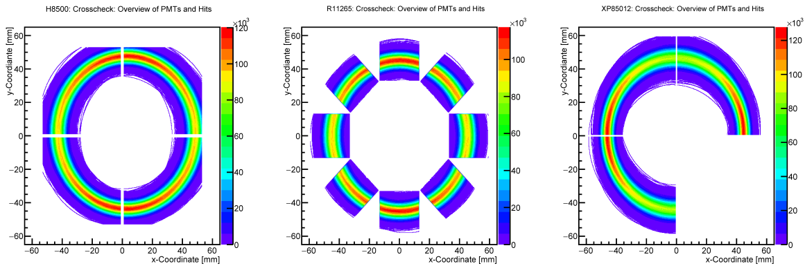
Figure 5.7. – As a crosscheck of the simulations all points lying on a sensor have been drawn (this excludes points in between two sensors and beneath the sensors) (left: H8500, mid: R11265, right: XP85012). The different behaviour in the ring mean range (i.e. the red colored area) is a result of the squared binning of the histograms.
