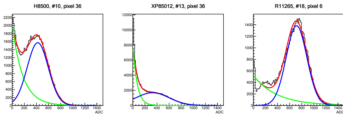
Figure 5.2. – Resulting fit distributions of the single-photon spectra of three single pixel for each sensor (left: H8500, PMT #10, pixel 36, middle: XP85012, PMT #13, pixel 36, right: R11265, PMT #18, pixel 6). Black remarks the data taken, red is the fitted sum functions consisting of an exponential part and a Gaussian and green (exponential) and blue (Gaussian) illustrate the separate parts. Larger differences in the result are visible for the R11265 MAPMT at low ADC values, as the second peak is not included in the fit function.
