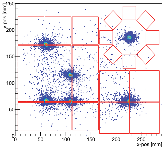
Figure 5.5. – Distributions of ring centers from the circle fit. Basis is the beamtest data (threshold scan 2), runs #176 - #181. Shown are ring positions A, B, D, E, G, and I.
