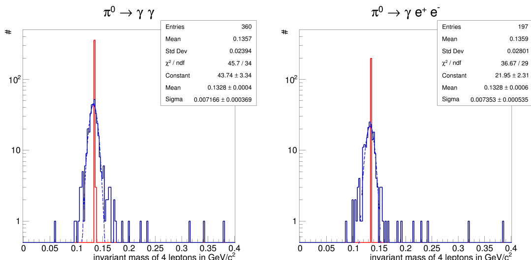
Figure 6.9. – Invariant mass of four electrons/positron from the same \pi^0 , identified with MC-true data, here separated by the two main decay-channels \pi^0 \rightarrow \gamma\gamma (left) and \pi^0 \rightarrow \gamma e^+e^- (right). The blue entries remark the combination with the reconstructed momenta, the red entries the combination with the MC-true momenta. The dashed blue line is a Gaussian fit of the combination with reconstructed momenta.
