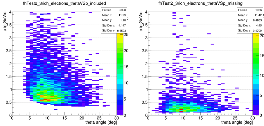
Figure 7.17. – Distribution of emission angles \theta of an electron versus its momentum p . Left: results for the three identified electrons of a \pi^0 , right: results for the unidentified electron of a \pi^0 .
