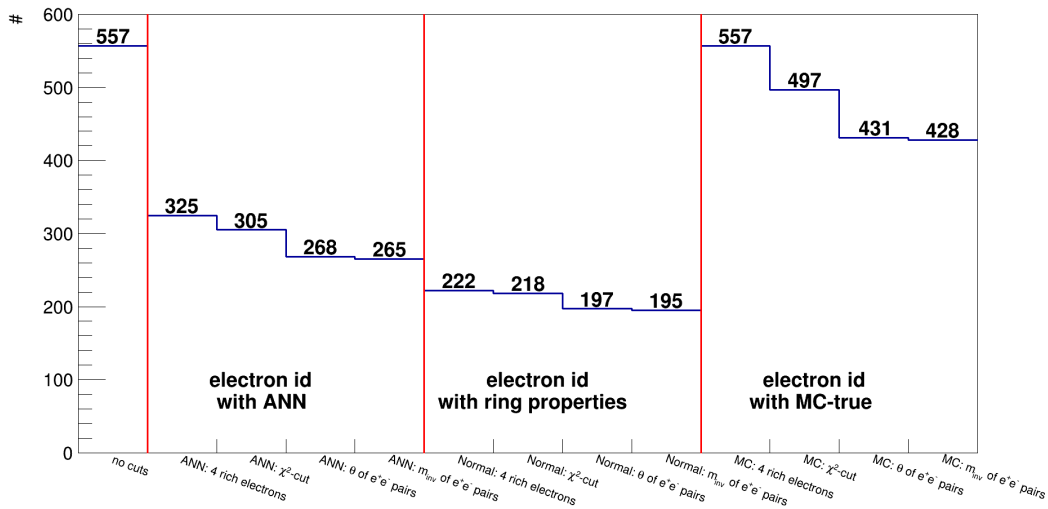
Figure 6.11. – Efficiency studies for the cuts derived in Section 6.6 for three different methods of electron identification (ANN, ring properties, MC-true). The cuts ( \chi^2 , opening angle \theta , and invariant mass m_{inv} of the e^+e^- -pairs) are applied consecutively and their effect on the number of reconstructed \pi^0 is shown.
