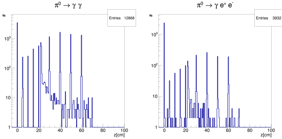
Figure 6.14. – Origins of electrons along the z -axis used for reconstruction of \pi^0 with the combined method, separated by the two main decay channels \pi^0 \rightarrow \gamma \gamma \rightarrow e^+ e^- e^+ e^- (left) and \pi^0 \rightarrow \gamma e^+ e^- \rightarrow e^+ e^- e^+ e^- (right). Included are conversion of the decay-photons only within the target ( \rightarrow reconstruction of 557 \pi^0 ) and also within the detector material ( \rightarrow reconstruction of 3643 \pi^0 ).
