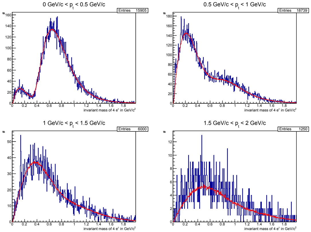
Figure 7.7. – Invariant mass spectra (blue) for different p_t -ranges between p_t = 0 \text{ GeV}/c and p_t = 2 \text{ GeV}/c . In red the scaled background spectra as calculated with EMT are shown. In each case the background fits very good to the signal spectrum.
