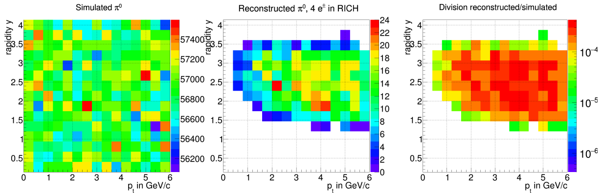
Figure 7.19. – Coverage of the phase-space in terms of transversal momentum p_t and rapidity y . Left: all simulated \pi^0 , mid: all reconstructed \pi^0 from the combined method, i.e. all four leptons identified in the RICH, right: ratio of reconstructed and simulated distribution.
