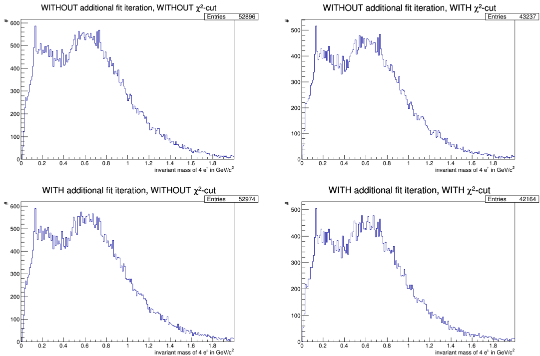
Figure 7.1. – Reconstructed invariant mass spectra for four different cases of applied cuts: without and with an additional fit iteration of the momentum fit (top/bottom), and without and with a cut on the \chi^2 of the momentum fit (left/right). For better visibility the binwidth was set to 10 \text{ MeV}/c^2 .
