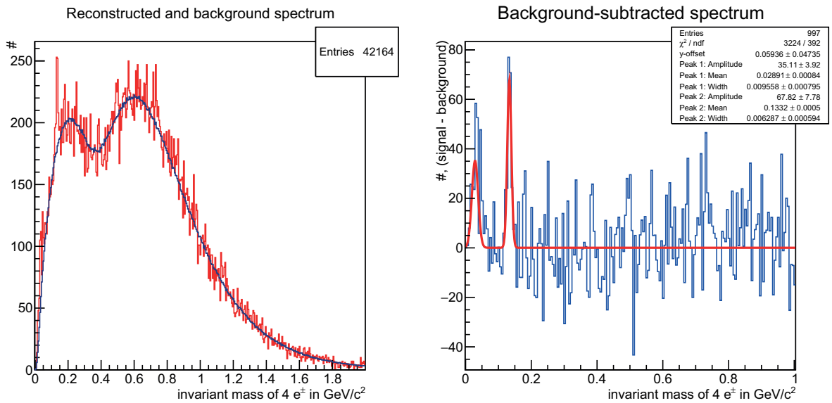
Figure 7.4. – Left: reconstructed invariant mass spectrum from the combination of 4 e^\pm (red) and the scaled background calculated with the event mixing technique (blue). Right: background-subtracted invariant mass spectrum (blue) with a double Gaussian fit for the \pi^0 -peak and the peak at very low invariant masses. The binwidth here is 5 \text{ MeV}/c^2 .
