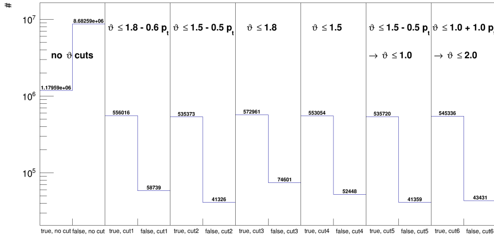
Figure 6.21. – Number of true and false combinations of e^+ and e^- to a photon (identified via MC-true). The numbers are given without any \vartheta -cut and also for the 6 different \vartheta -cuts given in the text. The above chosen \chi^2 -cut was included for all cases here.
