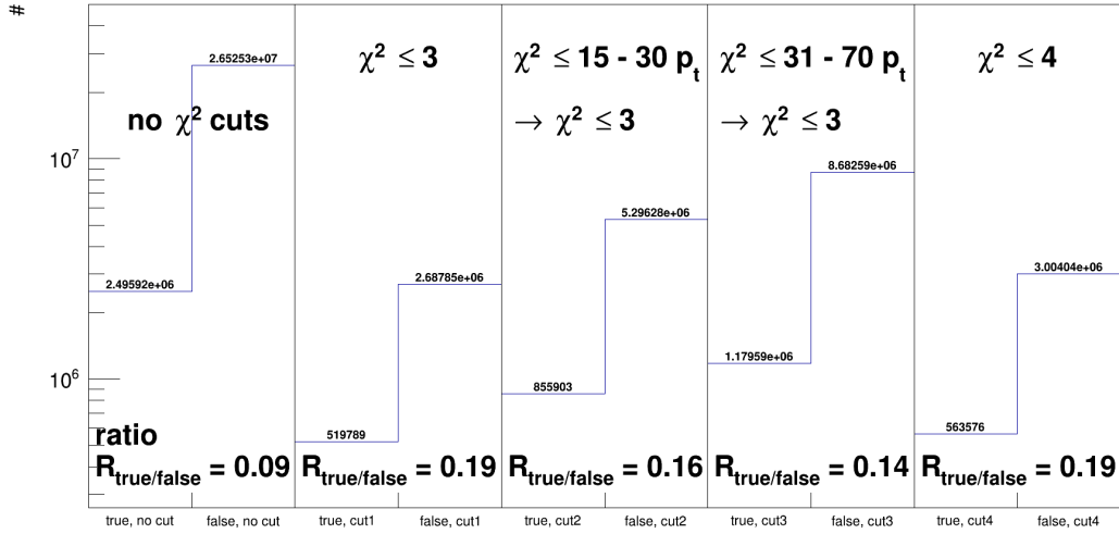
Figure 6.18. – Number of true and false combinations of e^+ and e^- to a photon (identified via MC-true). The numbers are given without any \chi^2 -cut and for the 4 different \chi^2 -cuts given in the text.
