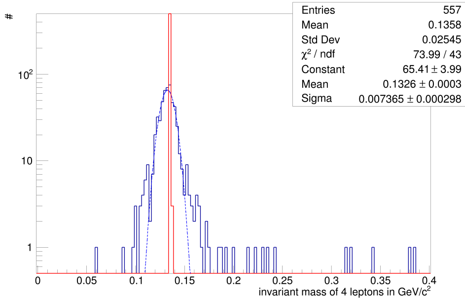
Figure 6.8. – Invariant mass of four electrons/positron from the same \pi^0 , identified with MC-true data. The blue entries remark the combination with the reconstructed momenta, the red entries the combination with the MC-true momenta. The dashed blue line is a Gaussian fit of the combination with reconstructed momenta.
