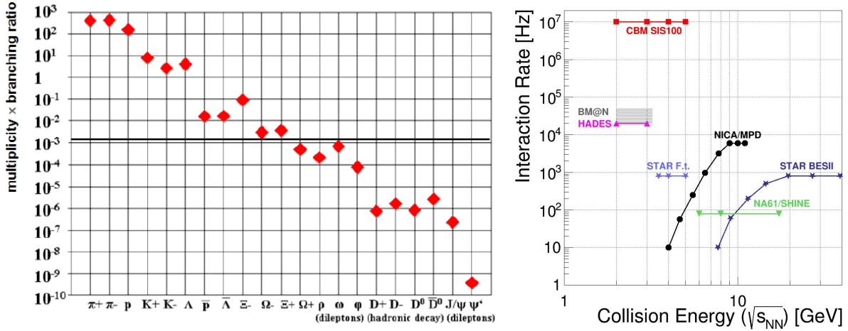
Figure 2.2. – Multiplicity times branching ratio for several rare probes (left, from [6]). The black horizontal line indicates those already measured (above) and those not yet measured (below). The right picture shows the interaction rate for several heavy-ion experiments (from [3]).
