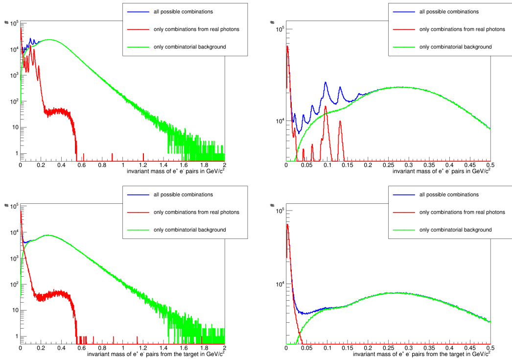
Figure 6.22. – Invariant mass distributions of electron-positron pairs. Blue: all possible combinations of electrons and positrons, red: only combinations originating from the same photon, green: only false combinations. Left shows the invariant mass range up to 2 \text{ GeV}/c^2 , the right picture shows a shorter range up to 0.5 \text{ GeV}/c^2 for better visibility. Both top pictures show all results, both bottom pictures the results only for leptons originating from the target. The comparison shows that the peaks at low invariant masses stem from photons converting in the detector material.
