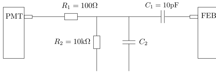
Figure 4.4. – Circuit diagram of attenuator board used for attenuating the signals from the sensors.
