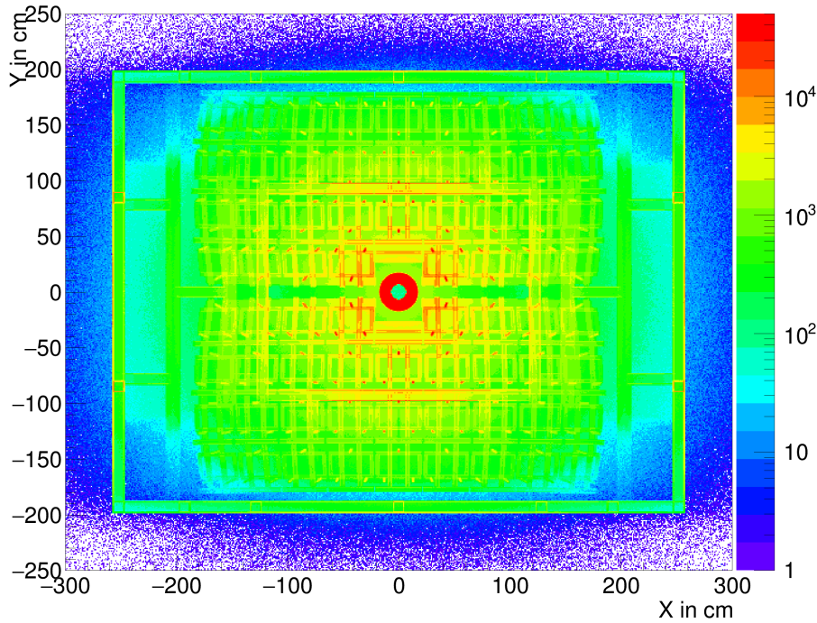
Figure 6.2. – Detector tomography of the CBM detector for the SIS100 setup. As basis 5 \cdot 10^6 UrQMD events were taken. The colour scale of this plot was cut off at higher values for better visibility of the different structures in the detector. Shown here is the x-y-projection of the region of the RICH detector, with applying a cut on the z-axis of 170 \text{ cm} \leq z \leq 400 \text{ cm} .
