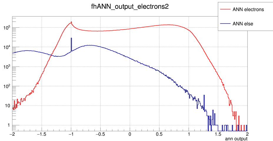
Figure 6.15. – Output from the ANN for electrons (red) and all other particles (blue), which make a signal in the RICH detector. The discrete spike at -1 is artificially generated and is a result from a not reconstructible ring.
