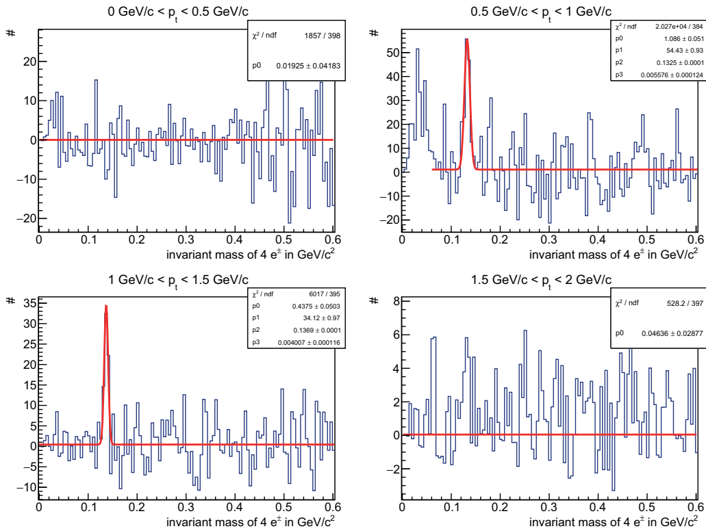
Figure 7.8. – Background-subtracted invariant mass spectra for different p_t -ranges (blue). In red fits of these spectra are shown. As fit function either a constant (first and fourth p_t -range) or a constant plus Gaussian (second and third p_t -ranges) were used.
