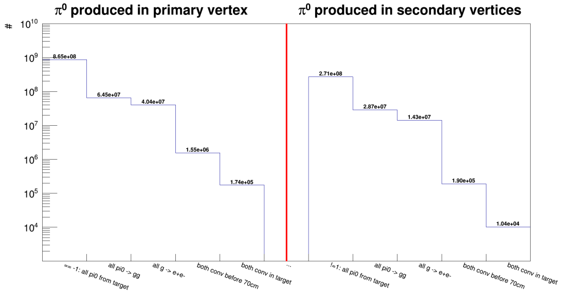
Figure 6.5. – Number of \pi^0 in the MC-true trackbank separated by their production within the primary vertex and within secondary vertices. Numbers are given for all \pi^0 produced (first column), all \pi^0 \rightarrow \gamma\gamma with both \gamma being in the trackbank (i.e. the \gamma or at least one of the e^\pm from conversion hit a detector; second column), all \pi^0 \rightarrow \gamma\gamma \rightarrow e^+e^-e^+e^- with all leptons being in the trackbank (third column), all conversions happening before z = 70 cm (fourth column), and all conversions happening in the target (fifth column). The numbers are slightly distorted as conversion within support structures and the magnet is also included, which can not be detected.
