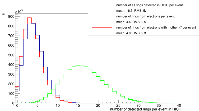
Figure 6.7. – Number of detected rings in the RICH detector for a simulation sample of 5 million central Au + Au collisions at 10 AGeV. Green: all detected rings; blue: rings from electrons, which have also a signal in the STS; red: rings from electrons, stemming from a \pi^0 , with a signal in the STS.
