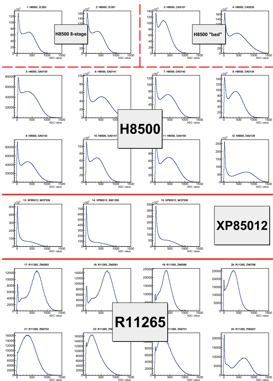
Figure 5.1. – Single-photon sum spectra of all 23 sensors used during the beamtest. The different models are indicated as also some ‘non-standard’ versions of the H8500 PMT are. These spectra only include the data from run #207 without any corrections.
