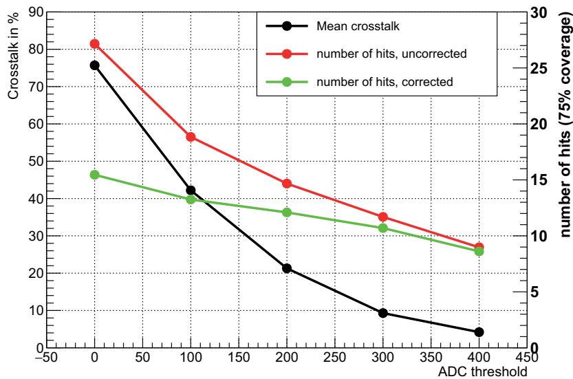
Figure 5.19. – Behaviour of the data for the Photonis XP85012 MCPs in terms of number of hits per ring for different applied ADC cuts. Black: development of crosstalk amount, red: mean number of hits per ring (without corrections for geometrical coverage, temperature, pressure, and crosstalk). green: mean number of hits per ring with crosstalk correction.
