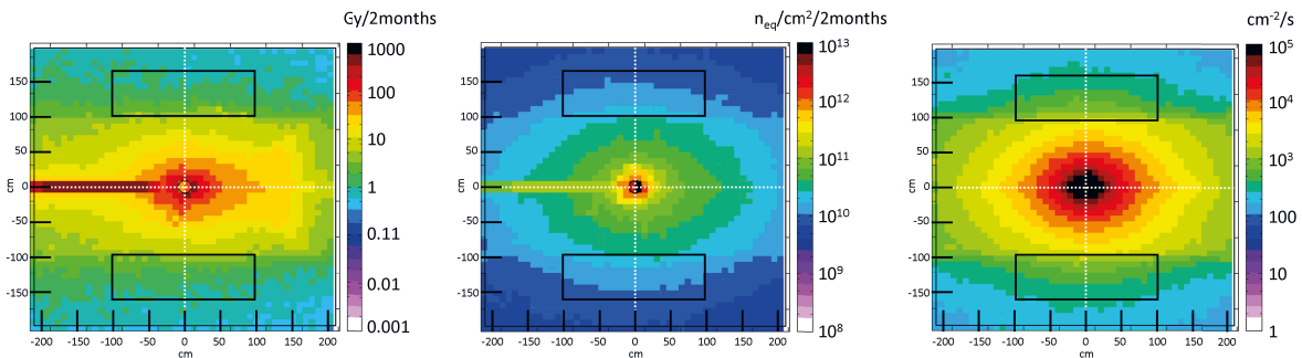
Figure 3.2. – Radiation environment for the RICH photon detector plane: Ionisation dose in Gy per 2 months (left), NIEL in n_{eq}/cm^2/2months (mid), high-energy hadron fluences in 1/cm^2/s (right). Plots correspond to approx. 5 \cdot 10^{15} beam particles, i.e. 2 months of CBM running with beam intensities of 10^9 ions/s. The photodetector position is indicated in the figures: Lower and upper edge of the photodetector are at \pm 97.5 cm and \pm 157.5 cm respectively. Vertical dimensions are \pm 1 m. (from [18]).
