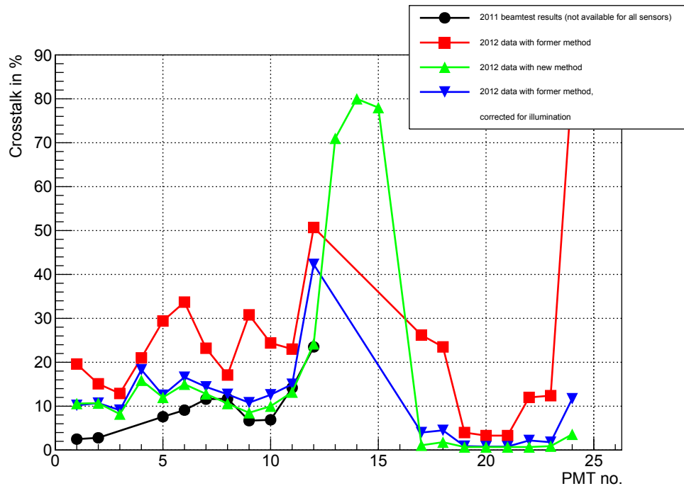
Figure 5.15. – Calculated crosstalk results from the beamtest 2012 gained from run #207 with the new enhanced method (green), with the old method (red), with the old method and applied corrections (blue), and results previously gained during the 2011 beamtest (black).
