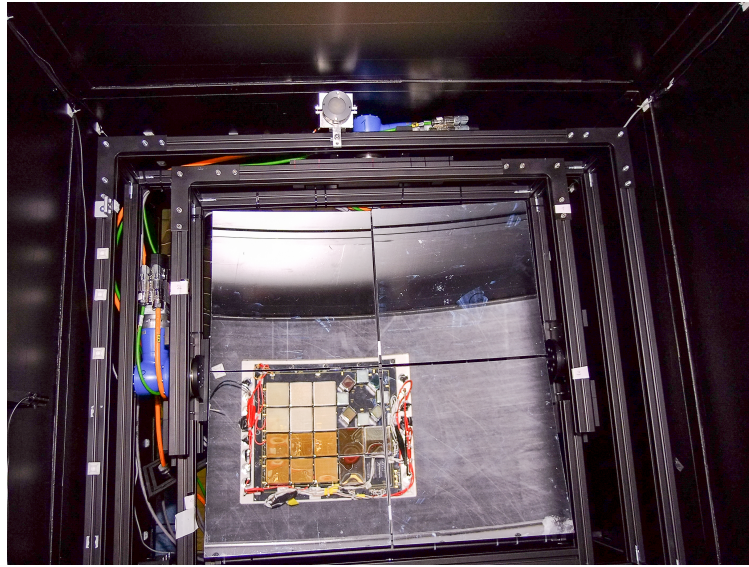
Figure 4.2. – Installed mirror frame holder inside the CBM-RICH prototype with the light pulser system on top of the frame. Visible is only the diffuser mounted inside a plastic tube. A picture of the photon camera can be seen in the mirror.
