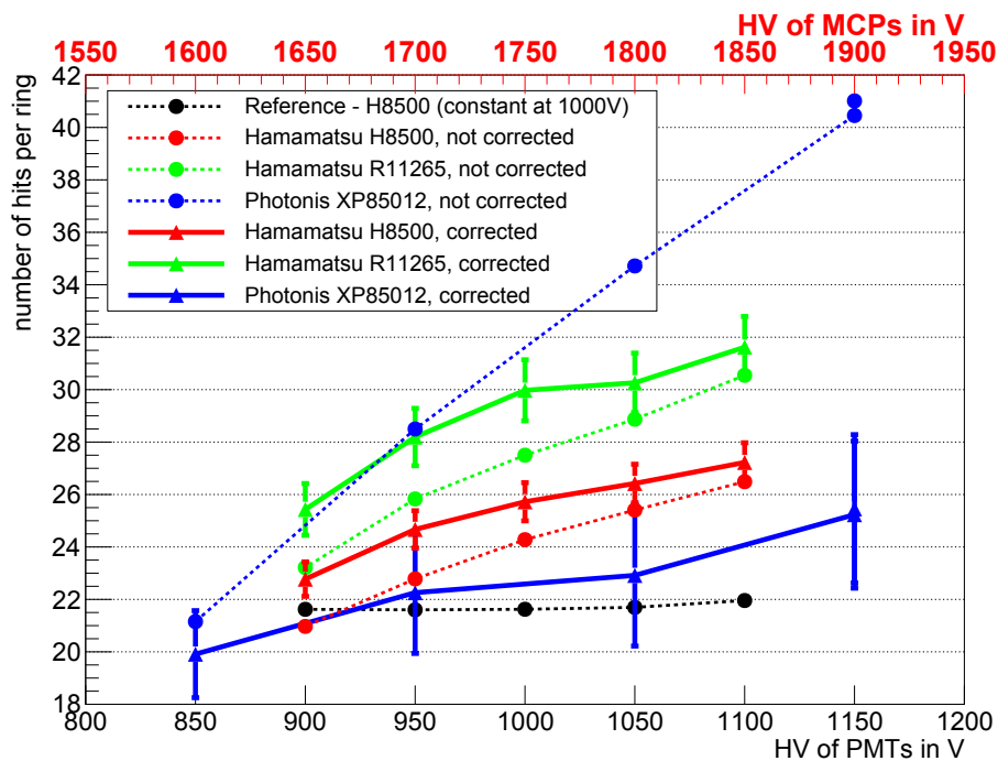
Figure 5.17. – Results for the number of detected hits per electron Cherenkov ring from the high-voltage scan. The high-voltage on positions I (Hamamatsu R11265), G (Photonis XP85012), and E (Hamamatsu H8500) was varied, and on position A (Hamamatsu H8500) was at a constant value for reference. The dashed lines remark the results with the correction of the geometrical coverage only, the continuous line with all applied corrections. The drawn error bars mark the uncertainty region based on the uncertainty of the calculated crosstalk.
