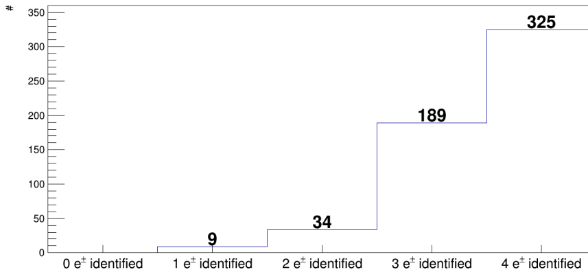
Figure 6.12. – Number of \pi^0 from which 0, 1, 2, 3, and all 4 electrons are identified based on the ANN and a cut-value of -0.8 . For most \pi^0 all four leptons are correctly identified with this cut (325). From the non-reconstructible \pi^0 (totally 232) mainly one of the four leptons was not correctly identified (189).
