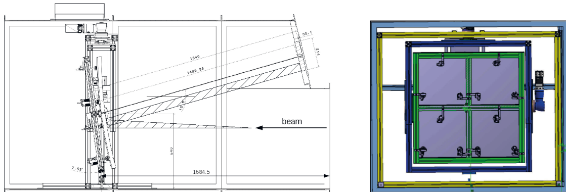
Figure 4.1. – Left: Technical drawing of the CBM-RICH prototype box with mirrors on a rotatable frame. The photon detector is mounted on the upper right side, above the beam entry. The hatched area visualizes the Cherenkov cone and its reflection onto the photon detector. Right: The mirror system. Each mirror tile is adjustable at three points. From [18].
