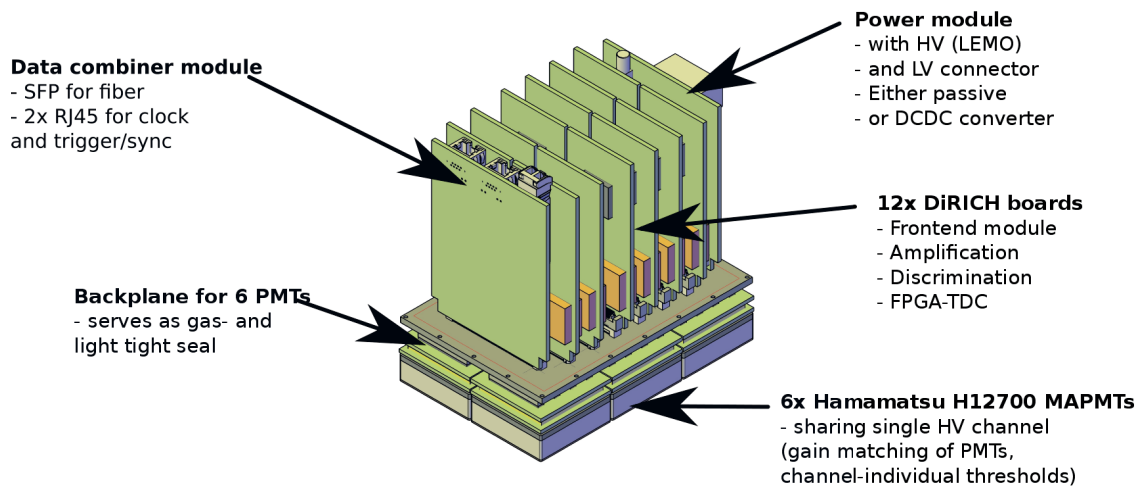
Figure 2.5. – Schematic layout of one camera module for the CBM-RICH camera, designed to carry 6 MAPMTs. It consists of 12 DiRICH modules (2 per sensor), one power module, and one data combiner module, all developed as plug-in devices on the PCB backplane.
