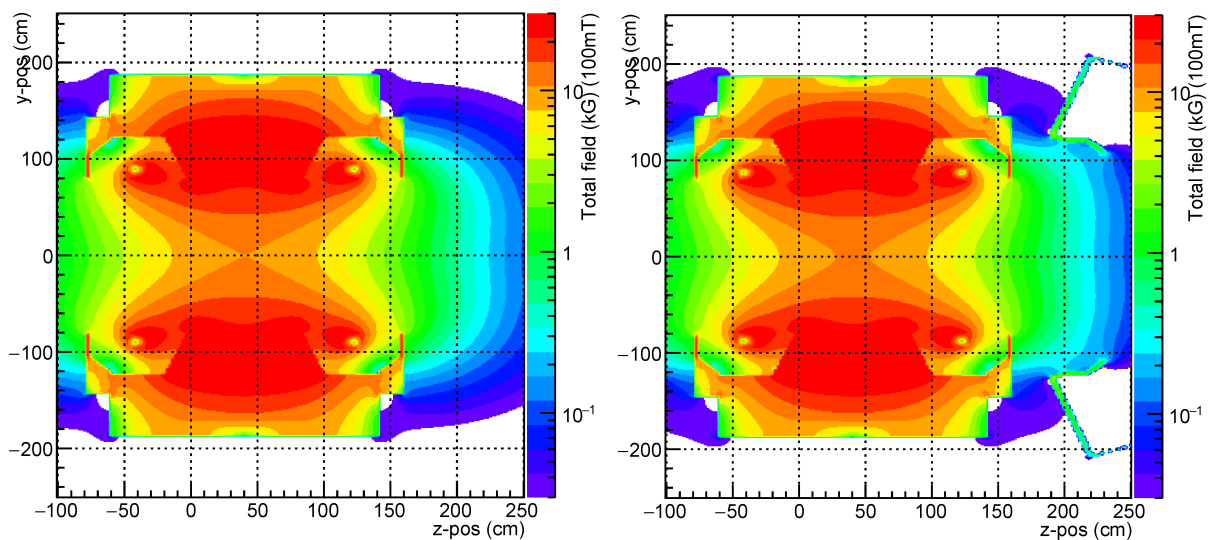
Figure 3.3. – Effects of a shielding box around the sensor camera of the CBM-RICH. The left picture visualizes the magnetic field strength in the region of magnet/MVD/STS and the front parts of the RICH without the shielding box, in the right picture the shielding box is included (clearly visible on the upper right and lower right part). With the shielding box the magnetic field strength in the region of the sensor camera is decreased to an acceptable value. (from [26])
