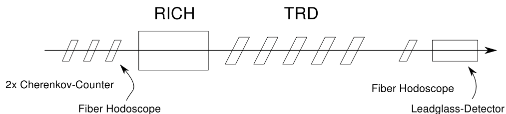
Figure 4.5. – Complete setup during the beamtest 2012. In the front two Cherenkov counters for particle identification and one fiber hodoscope for particle tracking were placed. The CBM-RICH prototype box and several CBM-TRD prototypes were arranged behind them. At last another fiber hodoscope for tracking and a leadglass detector for further particle identification were set up. The beam direction is indicated by a long arrow.
