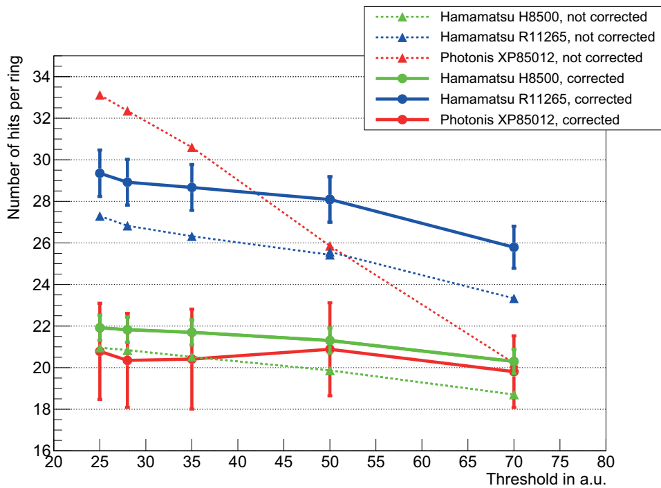
Figure 5.18. – Results for the number of detected hits per electron Cherenkov ring from the threshold scan. The dashed lines remark the results with the correction of the geometrical coverage only, the continuous line with all applied corrections. The drawn error bars mark the uncertainty region based on the uncertainty of the calculated crosstalk.
