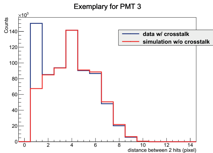
Figure 5.11. – Exemplary distance distribution for events containing exactly two hits, simulation (red) and data (blue). The simulation fits nearly perfectly in all bins except the first bin. This excess in the first bin can be explained by the amount of crosstalk (usually appearing in neighbouring pixel, i.e. at a distance of 1 or 1.4) in the data.
