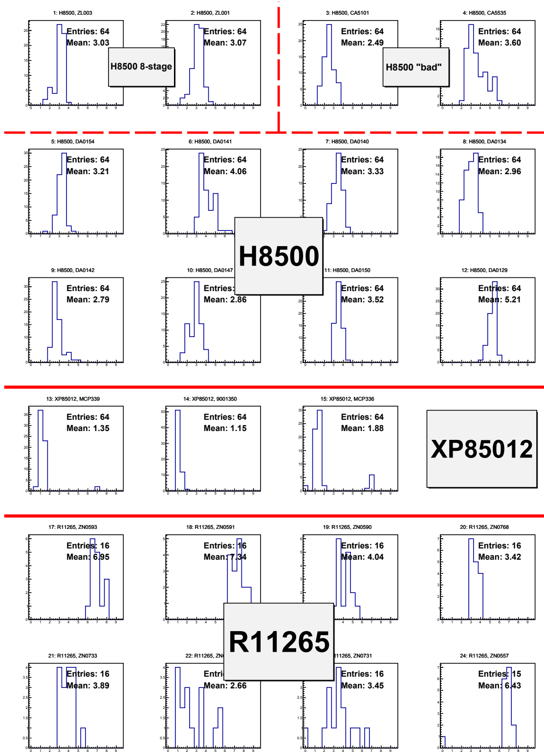
Figure 5.3. – Calculated gain values of all pixel for all sensors (in factors of 10^6 ).
