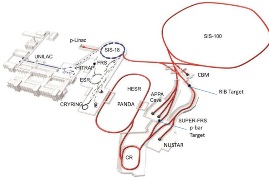
Figure 1.1. – Overview of all the existing GSI structures (on the left half, including the UNILAC and SIS18 accelerators in blue) and the new structure of FAIR (in red).
