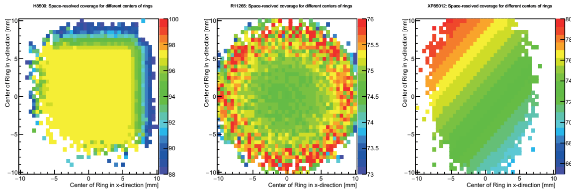
Figure 5.8. – Geometrical coverage as function of the simulated ring center (left: H8500, mid: R11265, right: XP85012). The different behaviour of the arrangements can clearly be recognized.
