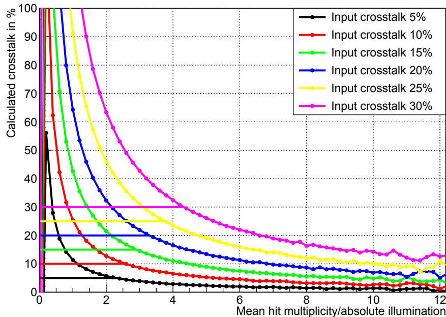
Figure 5.12. – Simulation of the behaviour of the old method of crosstalk calculation for different absolute illumination values and fixed input crosstalk values. Several simulations were done each with a fixed amount of crosstalk between 5% and 30%. Horizontal lines are additionally drawn (uo to the point, where the calculated crosstalk matches the input crosstalk) to indicate the input crosstalk value for each result.
