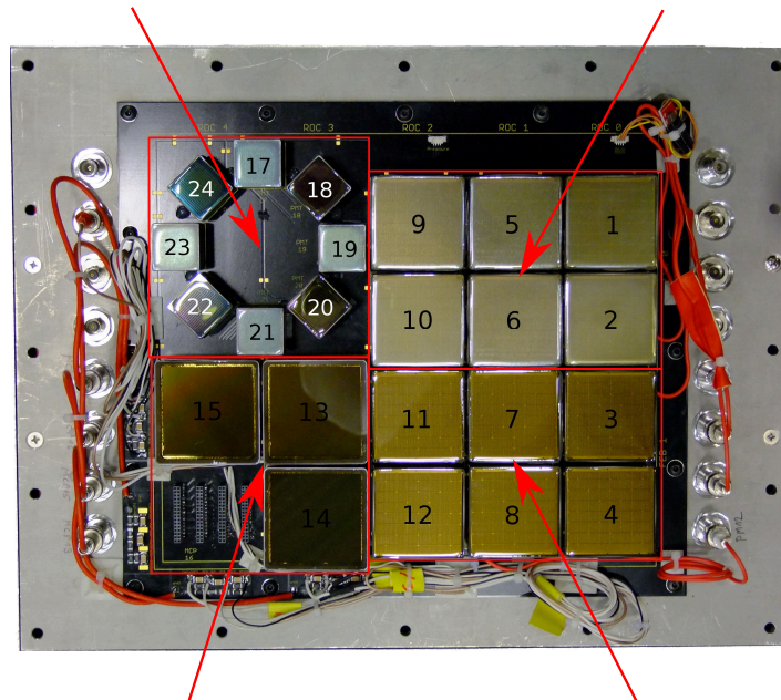
Figure 4.3. – CBM-RICH prototype camera during the beamtest 2012. The numbers indicate the position used in the analysis (compare Table 4.1).
