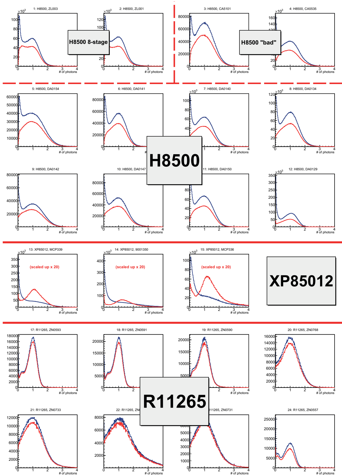
Figure 5.4. – Blue: normalized (to ‘number of photons’) and corrected (for pixel gain variations) single-photon sum-spectra of all 23 tested sensors. Red: resulting spectra only considering amplitude of hits, which do not have a hit in the 8 surrounding pixel. All spectra only include data from run #207.
