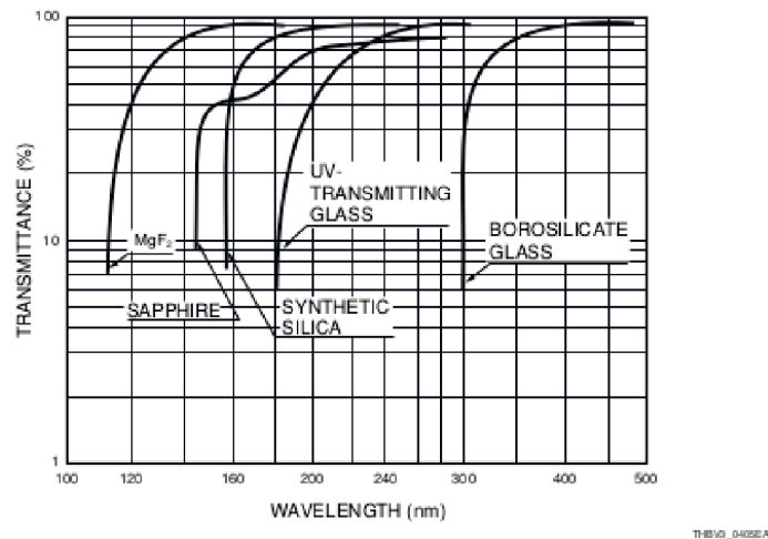
Figure 3.1. – Transmission curves of different photomultiplier window materials. (from [24]).
