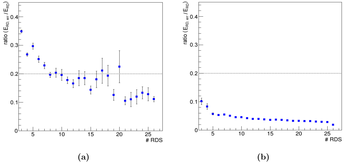
Figure 9.4: Ratio of RD Energy error to RD Energy versus number of RDS for the measured (a) and the simulated dataset (b).
