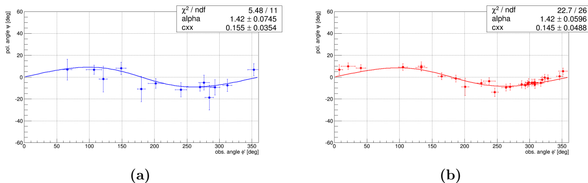
Figure 9.19: Polarization pattern of an air shower recorded under normal atmospheric field conditions from the measured (a) and simulated quality dataset (b).
