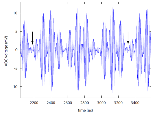
Figure 6.8: Voltage trace of the beacon beat after digital filtering has been applied. The period of the beat ( \sim 1.1 \mu\text{s} ) is indicated by the arrows. From [160].
