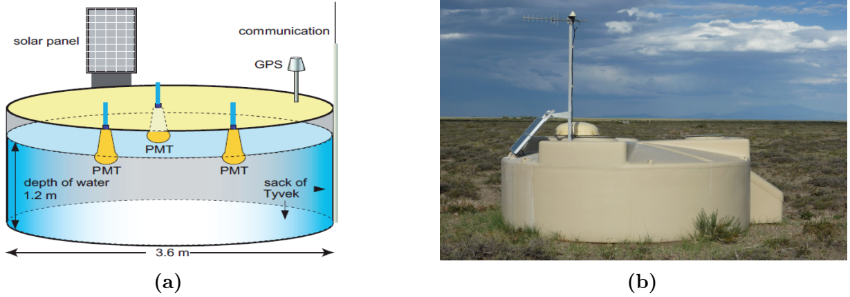
Figure 5.2: Schematic drawing of a Surface Detector Station (SDS) with its most important individual components [137] (a) and picture of a SDS within the Argentinean pampa (b).
