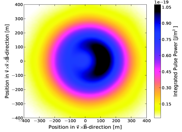
Figure 4.14: Interpolated two-dimensional pattern of the total pulse power in the shower plane for a simulated air shower ( \theta = 45^\circ , \phi = 37^\circ , E = 4.4 \times 10^{16} eV) showing the typical bean-shape pattern. From [83].
