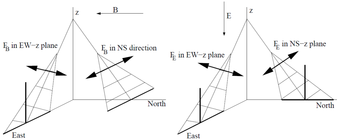
Figure 9.1: Schematic view of the direction of the magnetic (left) and electric (right) force and their influence on the polarization properties. Particle deflection is indicated by the arrows, the thick lines represent the pulse polarization. From [102].
