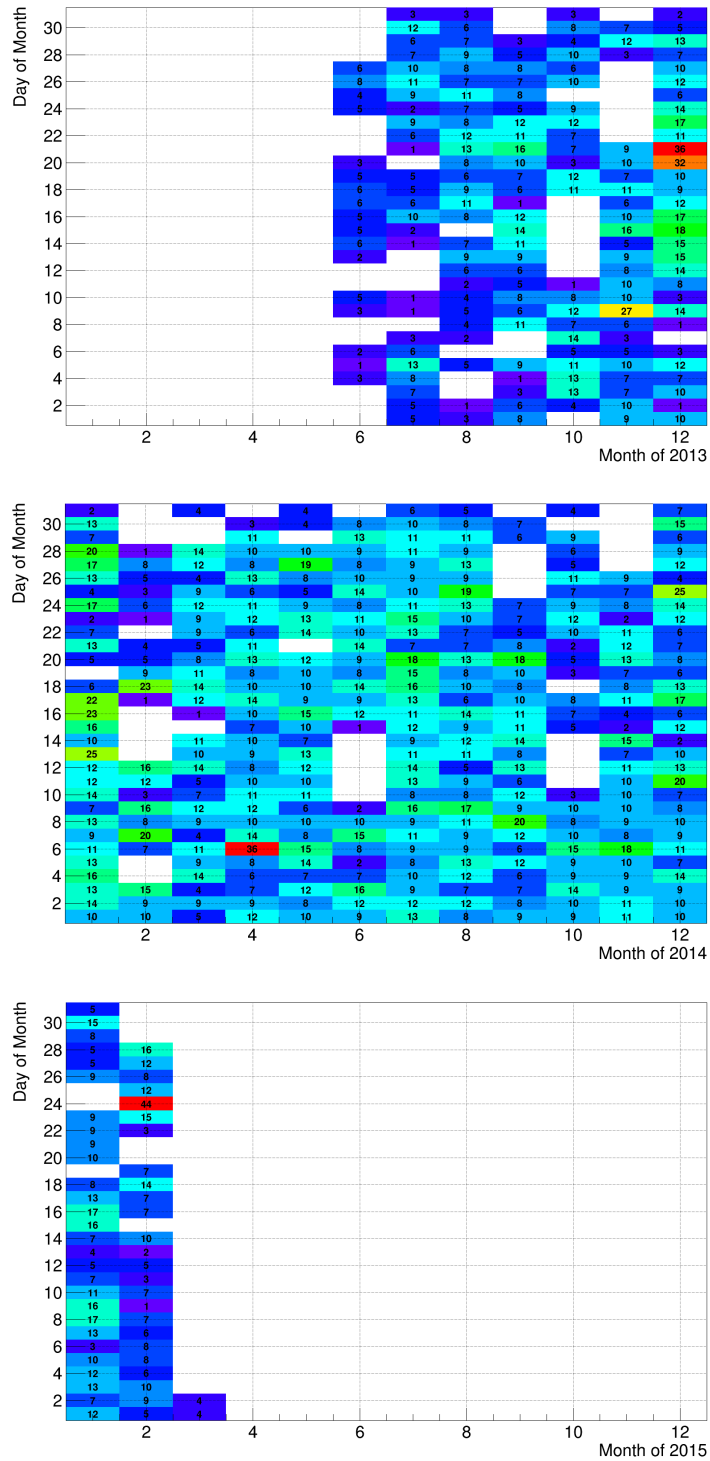
Figure 8.13: Annual maps (2013-2015) of the rate of reconstructed events for the full RdObserver v1r3 dataset.
