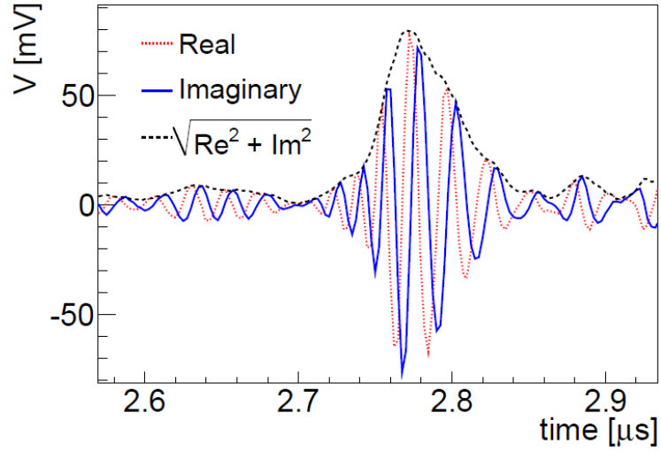
Figure 4.11: Example of a real time-series, the Hilbert transformed imaginary propagation and the calculated envelope. From [99].
