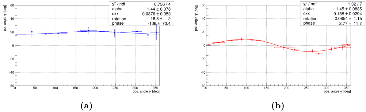
Figure 9.23: Polarization pattern of an air shower recorded under TS cond. from the measured dataset (a) and from the simulated dataset (b) with a fit of Eq. 9.6.
