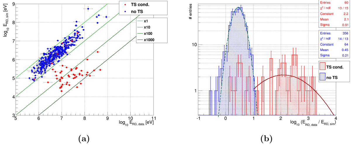
Figure 9.12: Radiated energies E_{RD, data} versus E_{RD, sim} (a) and ratio R(E_{RD, data}/E_{RD, sim}) (b) for the quality dataset. Events during TS cond. are marked in red, no TS in blue.
