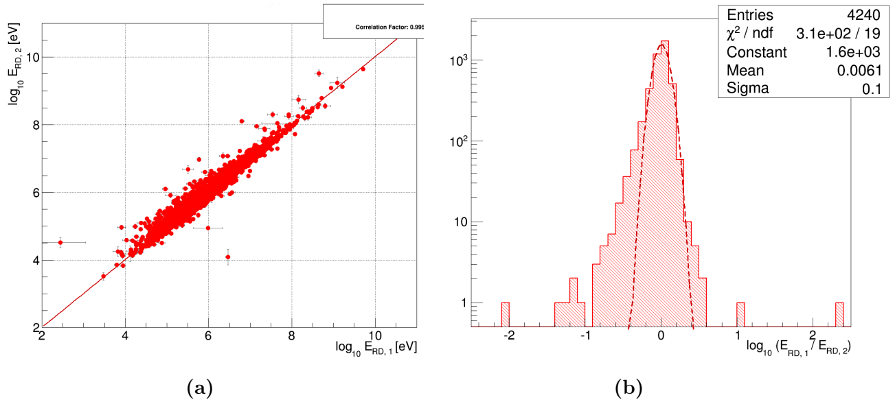
Figure 9.2: Comparison of the estimated radio energy for proton ( E_{RD,1} ) and iron ( E_{RD,2} ) simulations. Correlation plot (a) and ratio with Gaussian fit (b).
