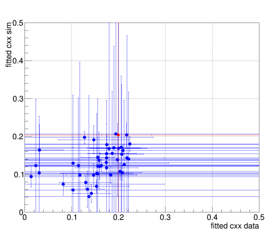
Figure 9.20: Correlation of the fitted charge-excess fraction a between the measured and simulated dataset. No TS (blue) and TS cond. (red).
