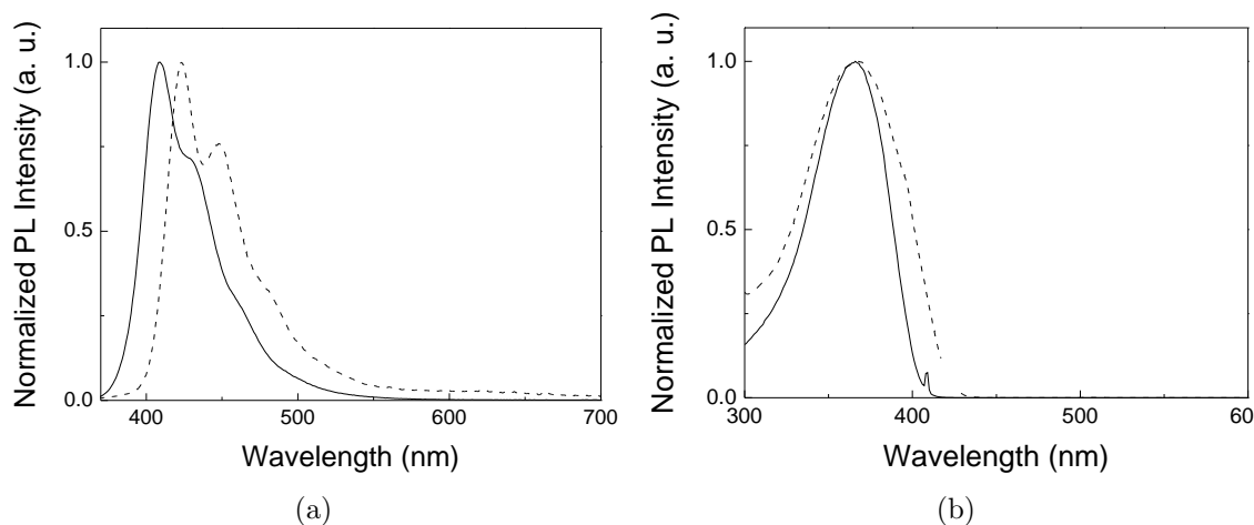
Figure 6.2.5: a) Emission and b) excitation spectra of PBS-PFP-PDI ( 5 \times 10^{-6} M) in the presence (dashed line) and absence (solid line) of PAH in water/dioxane (1:1, v/v) mixture.
