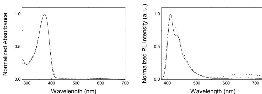
Figure 5.2.32: Absorption (left) and photoluminescence spectra (right) of PBS-PFP-TBTT 10 in water co-solvent mixtures. water/dioxane (solid line) and water/methanol (1:1, v/v) (dashed line).
