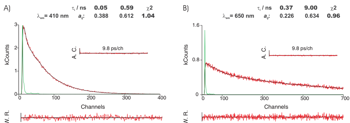
Figure 5.2.19: Fluorescence emission decay for PBS-PFP-DPP in 1 \times 10^{-4} M aqueous C_{12}E_5 obtained with \lambda_{exc} 372 nm at 298 K and collected at A) 410 nm and B) 650 nm. The green lines in the decays are the instrumental response function (IRF). For a better judgment of the quality of the fits weighted residuals (W.R., scale -3 \leq \sigma \leq +3 ) autocorrelation functions (A.C.) and chi-square values ( \chi^2 ) are also presented.
