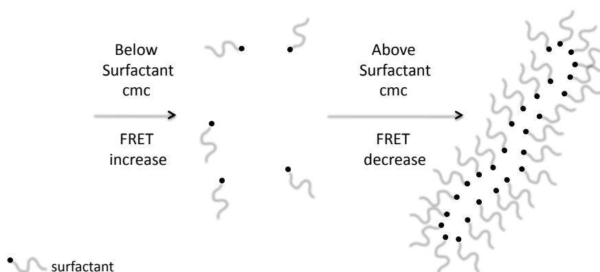
Figure 6.1.15: Schematic diagram that represents the predicted system constituents in three stages: pure copolymers emission, addition of surfactants, aggregation, and formation of copolymer+surfactant complexes.
