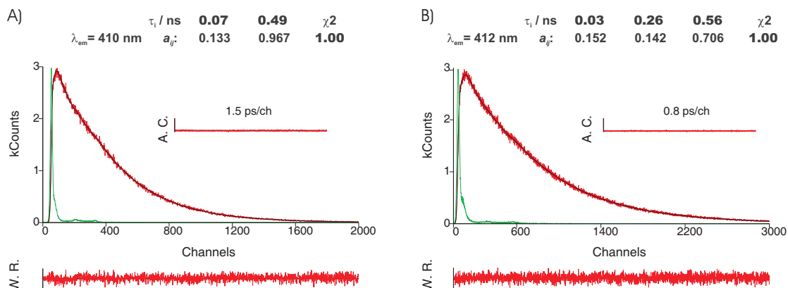
Figure 5.2.44: Fluorescence emission decay obtained with \lambda_{\text{exc}} 392 nm at 298.15 K in water/dioxane (1:1, v/v) mixture for A) PBS-PFP-TTP-TBTT collected at 410 nm and B) PBS-PFP collected at 412 nm. The green lines in the decays are the instrumental response function (IRF). For a better judgment of the quality of the fits weighted residuals (W.R., scale -3 \leq \sigma \leq +3 ), autocorrelation functions (A.C.) and \chi^2 are also presented.
