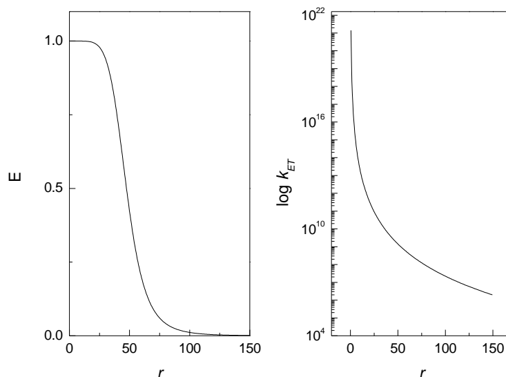
Figure 5.2.5: Dependence of the energy transfer efficiency ( E ) on the donor acceptor distance (left) and variation of the rate of energy transfer as a function of the donor acceptor distance for the PBS-PFP-PDI system (right).
