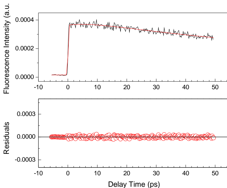
Figure 5.2.10: Femtosecond time resolved experiment of PBS-PFP-PDI in a water/dioxane (1:1, v/v) mixture. Excitation wavelength 370 nm and detection at 450 nm.
