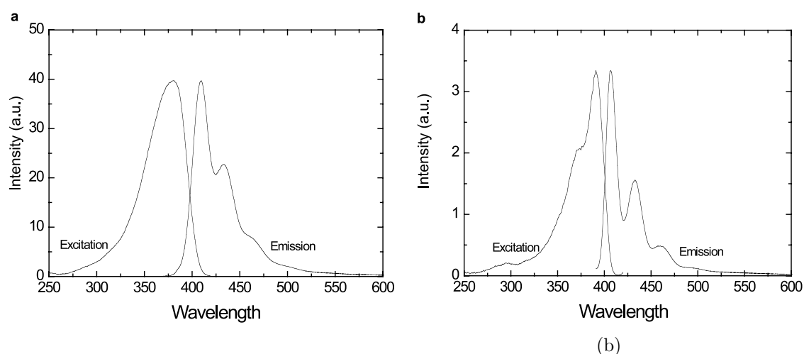
Figure 1.0.12: Excitation and emission spectra of PF2/6 in dilute methylocyclohexane solution at 295 K (a) and 77 K (b). Reproduced with permission from Ref. [43]. © (2008) Springer.
