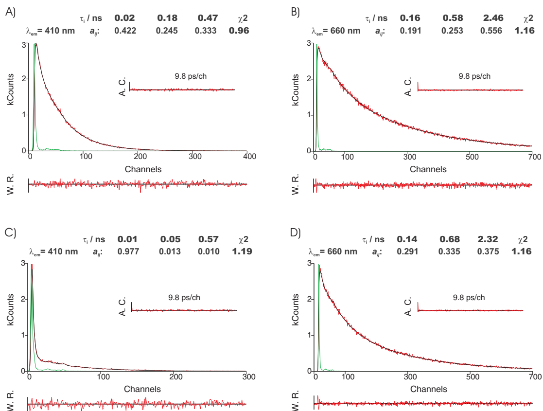
Figure 5.2.36: Fluorescence emission decay for PBS-PFP-TBTT 16 obtained with \lambda_{exc} 392 nm at 293 K and collected at PFP and TBTT emission maximum. A) and B) in water/dioxane (1:1, v/v) mixture. C) and D) in water/methanol (1:1, v/v) mixture. The green lines in the decays are the instrumental response function (IRF). For a better judgment of the quality of the fits weighted residuals (W.R., scale -3 \leq \sigma \leq +3 ) autocorrelation functions (A.C.) and chi-square values ( \chi^2 ) are also presented.
