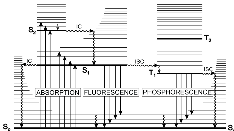
Figure 1.0.11: Perrin-Jablonski diagram showing the radiative and non-radiative transitions. S and T stands for the singlet and triplet state, respectively, IC stands for internal conversion and ISC for intersystem crossing. Reproduced with permission from Ref. [44]. © (2002) Wiley-VCH Verlag GmbH & Co. KGaA.
