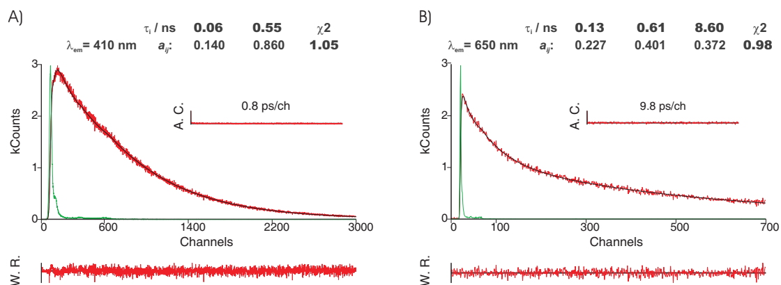
Figure 5.2.18: Fluorescence emission decay for PBS-PFP-DPP in water/dioxane (1:1, v/v) mixture obtained with \lambda_{exc} 372 nm at 298 K and collected at A) 410 nm and B) 650 nm. The green lines in the decays are the instrumental response function (IRF). For a better judgment of the quality of the fits weighted residuals (W.R., scale -3 \leq \sigma \leq +3 ) autocorrelation functions (A.C.) and chi-square values ( \chi^2 ) are also presented.
