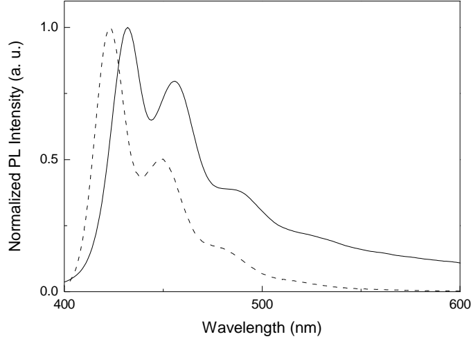
Figure 3.2.2: Normalized fluorescence spectra in thin film (solid line) and in NMP solution (dashed line).
