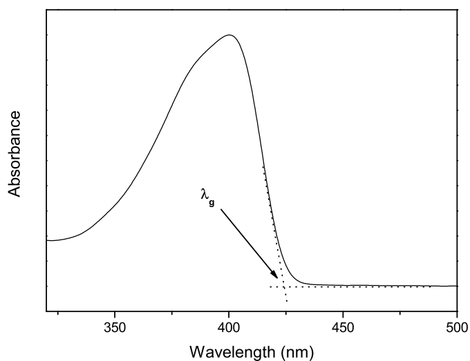
Figure 2.19.1: Band-gap determination via UV-vis spectra. Adapted from [40].
