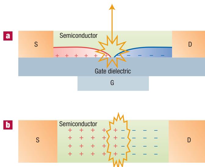
Figure 1.0.6: Scheme of a light-emitting field-effect transistor. Top: side view. Bottom: top view. The electrons and holes are injected from the drain (D) and source (S) contacts and recombine within the channel in a position controlled by the gate (G). Reproduced with permission from Ref. [3]. © (2006) Nature.
