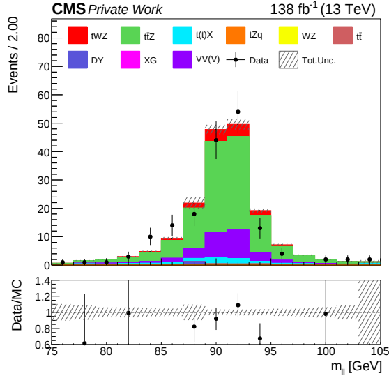
Figure 6.9: Distribution of the invariant mass of the dilepton pair with the closest invariant mass to the mass of the Z in the 4\ell SR for the Run 2 period. The black markers represent the data, while the solid stacked histogram shows the MC predictions for the various background processes. The dashed band indicates the total uncertainty. The lower panel displays the ratio between data and simulation.
