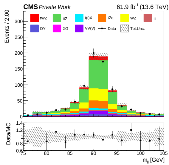
Figure 6.6: Distribution of the invariant mass of the dilepton pair with the closest invariant mass to the mass of the Z in the 3\ell SR for the Run 3 period. The black markers represent the data, while the solid stacked histogram shows the MC predictions for the various background processes. The dashed band indicates the total uncertainty. The lower panel displays the ratio between data and simulation.
