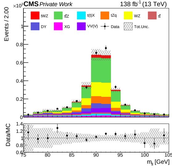
Figure 6.4: Distribution of the invariant mass of the dilepton pair with the closest invariant mass to the mass of the Z in the 3\ell SR for the Run 2 period. The black markers represent the data, while the solid stacked histogram shows the MC predictions for the various background processes. The dashed band indicates the total uncertainty. The lower panel displays the ratio between data and simulation.
