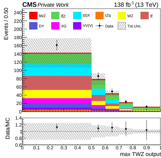
Figure 7.5: Max TWZ output distribution in the t\bar{t}X CR for Run 2 data. The black markers represent the data, while the solid stacked histogram shows the MC predictions for the various background processes. The dashed band indicates the total uncertainty. The lower panel displays the ratio between data and simulation.
