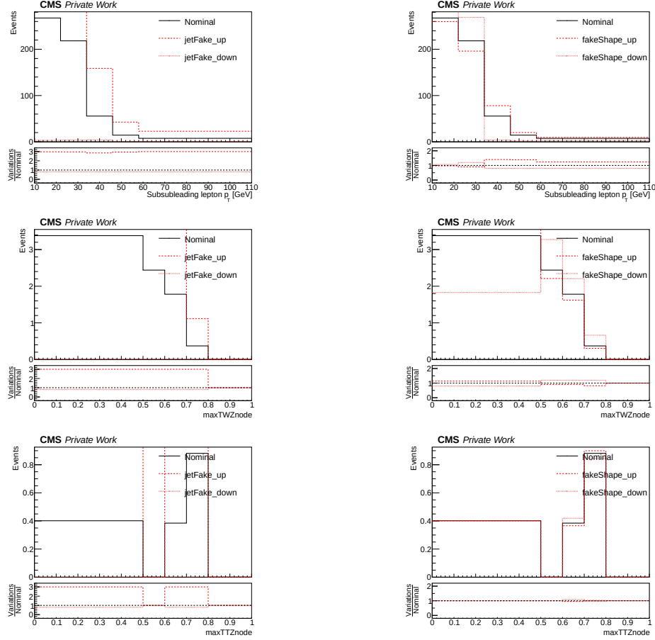
Figure A.28: Nominal event yields and fake lepton nuisances variations for the DY background in the 2022post data-taking year. The subsubleading lepton p_T , the \max TWZ output, and the \max TTZ output distributions are shown from the first to the last row. The subsubleading lepton p_T distribution is presented in the DY CR, while the ML output distributions in the 3\ell SR. The first column shows the templates of the jet fakes uncertainty, while in the second column the templates of the fakes shape nuisance is presented. The black line represents the nominal distribution, while the dotted red lines indicate the up and down variations. The range in the ratio plot is adjusted to display the entire distributions.
