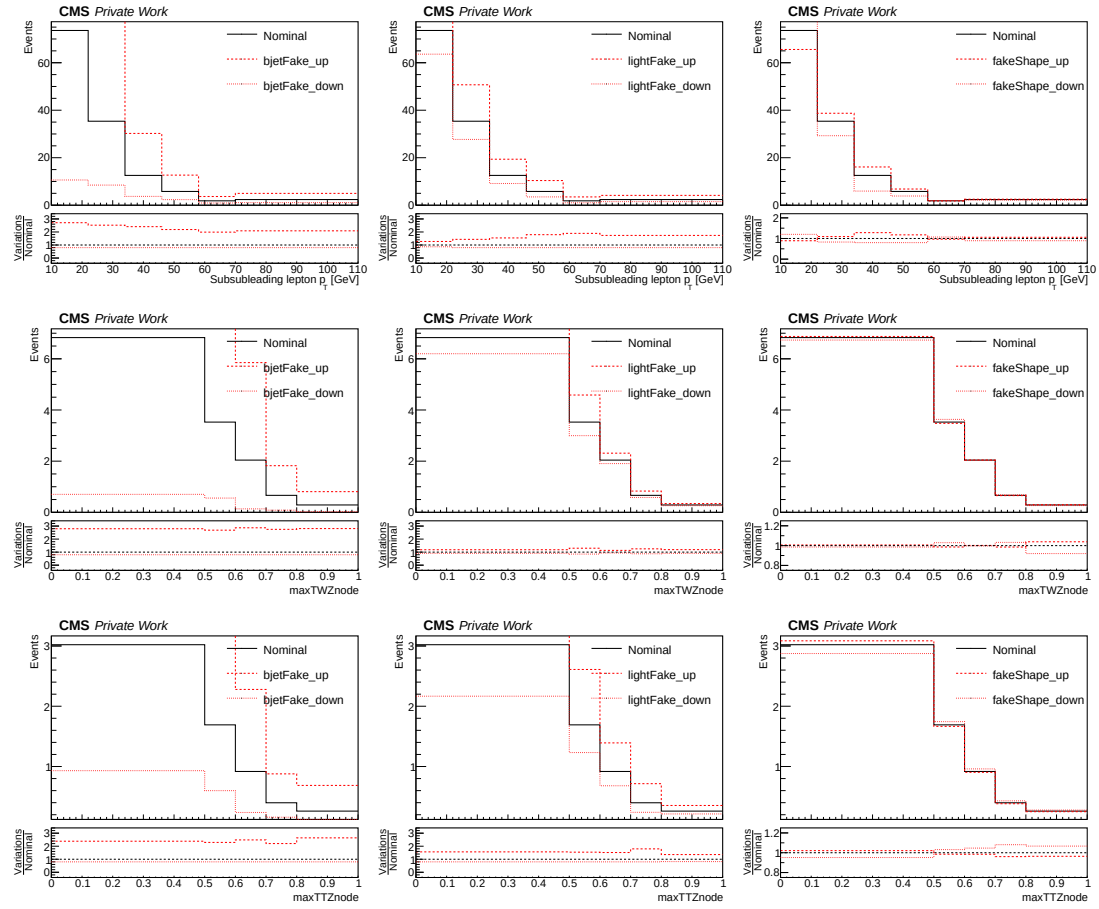
Figure A.23: Nominal event yields and fake lepton nuisances variations for the t\bar{t} background in the 2017 data-taking year. The subsubleading lepton p_T , the max\ TWZ output, and the max\ T\bar{T}Z output distributions are shown from the first to the last row respectively. In particular, the subsubleading lepton p_T distribution is shown in the t\bar{t}X control region, while the two ML output distributions correspond to the semi-leptonic signal region. The first two columns show the templates of the b -jets fakes and light -jets fakes uncertainties respectively, while in the third column the templates of the fakes\ shape nuisance is presented. The black line represents the nominal distribution, while the dotted red lines indicate the up and down variations. The range in the ratio plot is adjusted to display the entire distributions.
