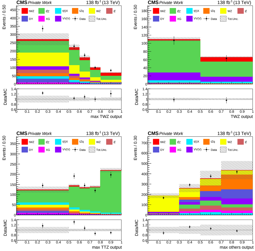
Figure A.33: Pre-fit distributions in the SRs for the fit on Run 2 data. The max TWZ output (top left), max TTZ output (bottom left), and max others output (bottom right) distributions are shown in the 3 \ell SR, while the tWZ ML output node distribution (top right) is shown in the 4 \ell SR. The black markers represent the data, while the solid stacked histogram shows the MC predictions for the various background processes. The dashed band indicates the total uncertainty. The lower panel displays the ratio between data and simulation.
