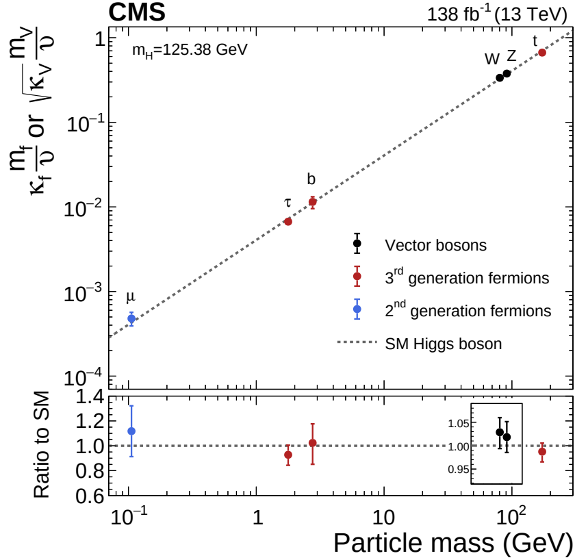
Figure 1.5: The measured coupling modifiers of the Higgs boson to fermions and heavy gauge bosons, as functions of fermion or gauge boson mass, where v is the vacuum expectation value of the Higgs field. For gauge bosons, the square root of the coupling modifier is plotted to keep a linear proportionality to the mass, as predicted in the SM. Taken from Ref. [32].
