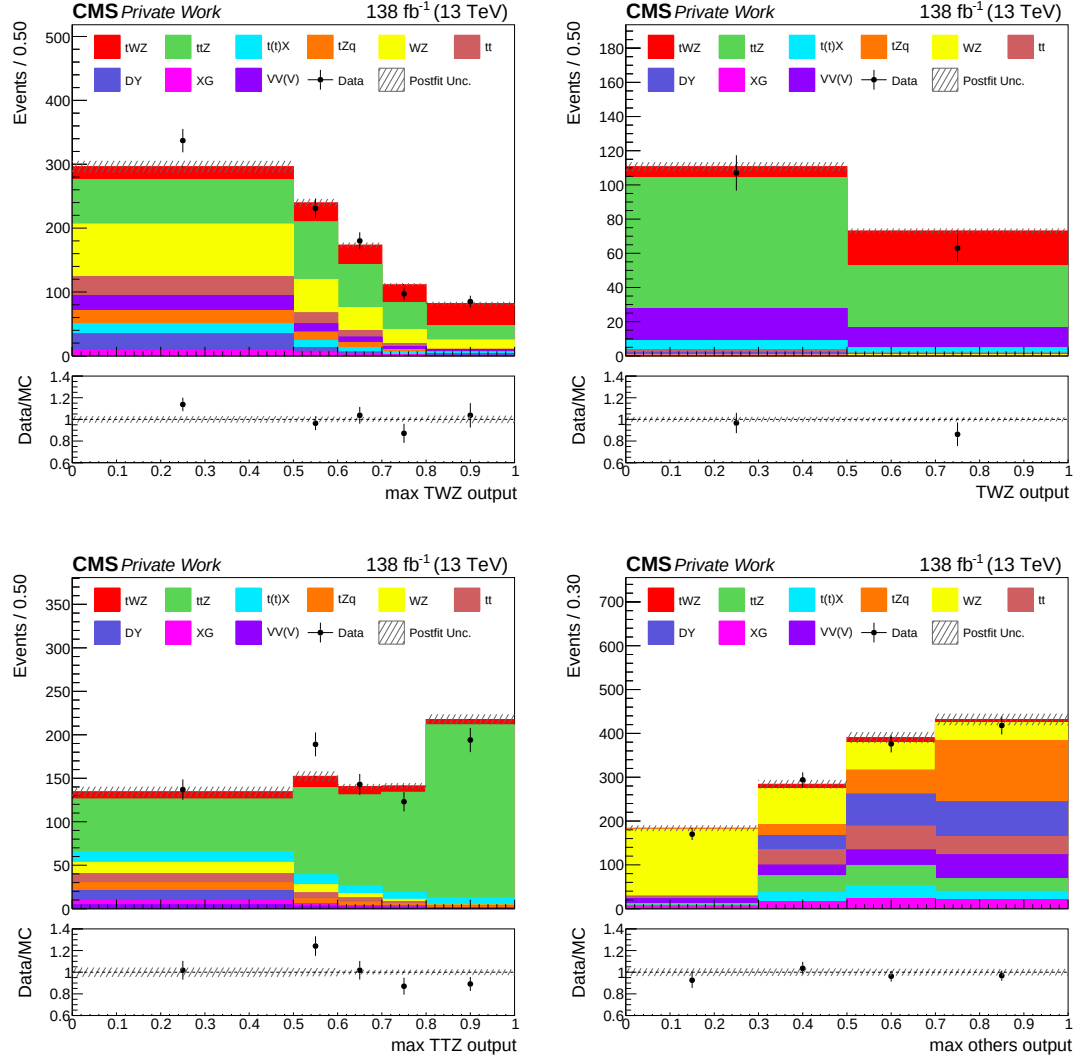
Figure 10.1: Post-fit distributions in the SRs for the fit on Run 2 data. The \max TWZ output (top left), \max TTZ output (bottom left), and \max others output (bottom right) distributions are shown in the 3\ell SR, while the tWZ ML output node distribution (top right) is shown in the 4\ell SR. The black markers represent the data, while the solid stacked histogram shows the MC predictions for the various background processes after the fit to data. The dashed band indicates the post-fit uncertainty. The lower panel displays the ratio between data and simulation.
