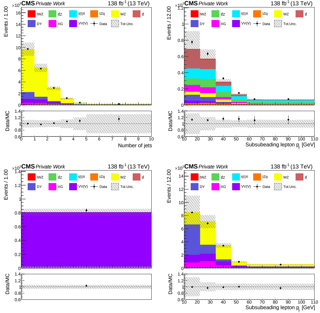
Figure A.34: Pre-fit distributions in the CRs for the fit on Run 2 data. The jet multiplicity distribution is shown in the WZ CR (top left), the event yields in the ZZ CR (bottom left), and the subleading lepton transverse momentum in the ttX CR (top right) and DY CR (bottom right). The black markers represent the data, while the solid stacked histogram shows the MC predictions for the various background processes. The dashed band indicates the total uncertainty. The lower panel displays the ratio between data and simulation.
