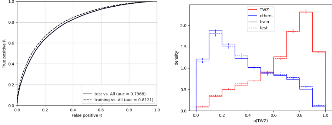
Figure 7.10: Left: ROC curves for the tWZ classification. The solid curve corresponds to the test-vs-all ROC, while the dashed curve shows the ROC for the training set. The AUC is reported in the legend for both cases. Right: Output node distributions of the 4\ell SR algorithm. For each class, the predicted probabilities are shown separately for the training (solid lines) and test (dashed lines) datasets. The colour indicates the true class of the events.
