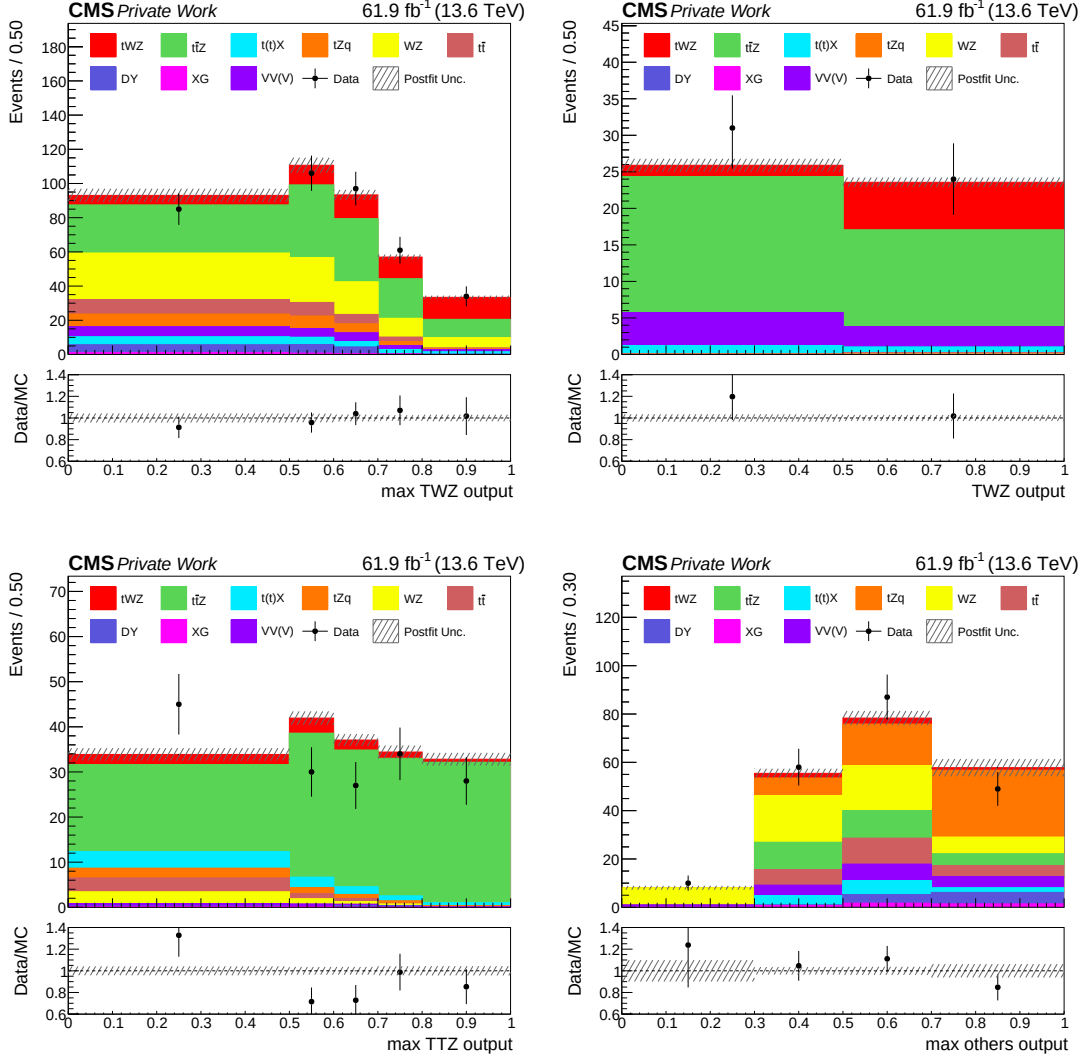
Figure 10.5: Post-fit distributions in the SRs for the fit on Run 3 data. The max TWZ output (top left), max TTZ output (bottom left), and max others output (bottom right) distributions are shown in the 3\ell SR, while the max TWZ ML output node distribution (top right) is shown in the 4\ell SR. The black markers represent the data, while the solid stacked histogram shows the MC predictions for the various background processes after the fit to data. The dashed band indicates the post-fit uncertainty. The lower panel displays the ratio between data and simulation.
