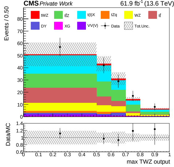
Figure 7.9: Max TWZ output distribution in the t\bar{t}X CR for Run 3 data. The black markers represent the data, while the solid stacked histogram shows the MC predictions for the various background processes. The dashed band indicates the total uncertainty. The lower panel displays the ratio between data and simulation.
