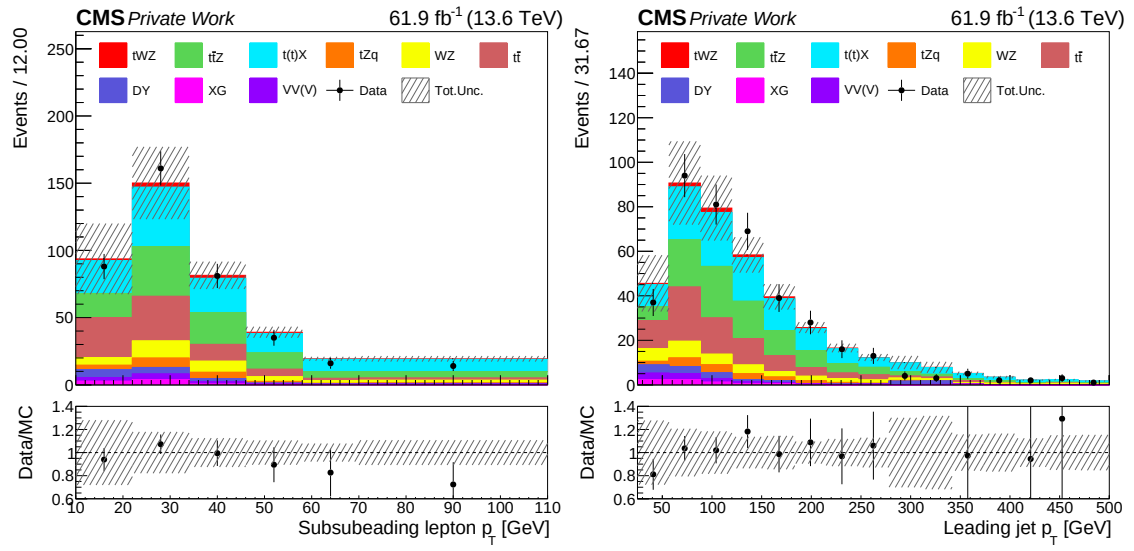
Figure 6.22: Distributions of the transverse momentum of the subsubleading lepton (left) and leading jet (right) in the t\bar{t}X CR for the Run 3 period. The black markers represent the data, while the solid stacked histogram shows the MC predictions for the various background processes. The dashed band indicates the total uncertainty. The lower panel displays the ratio between data and simulation.
