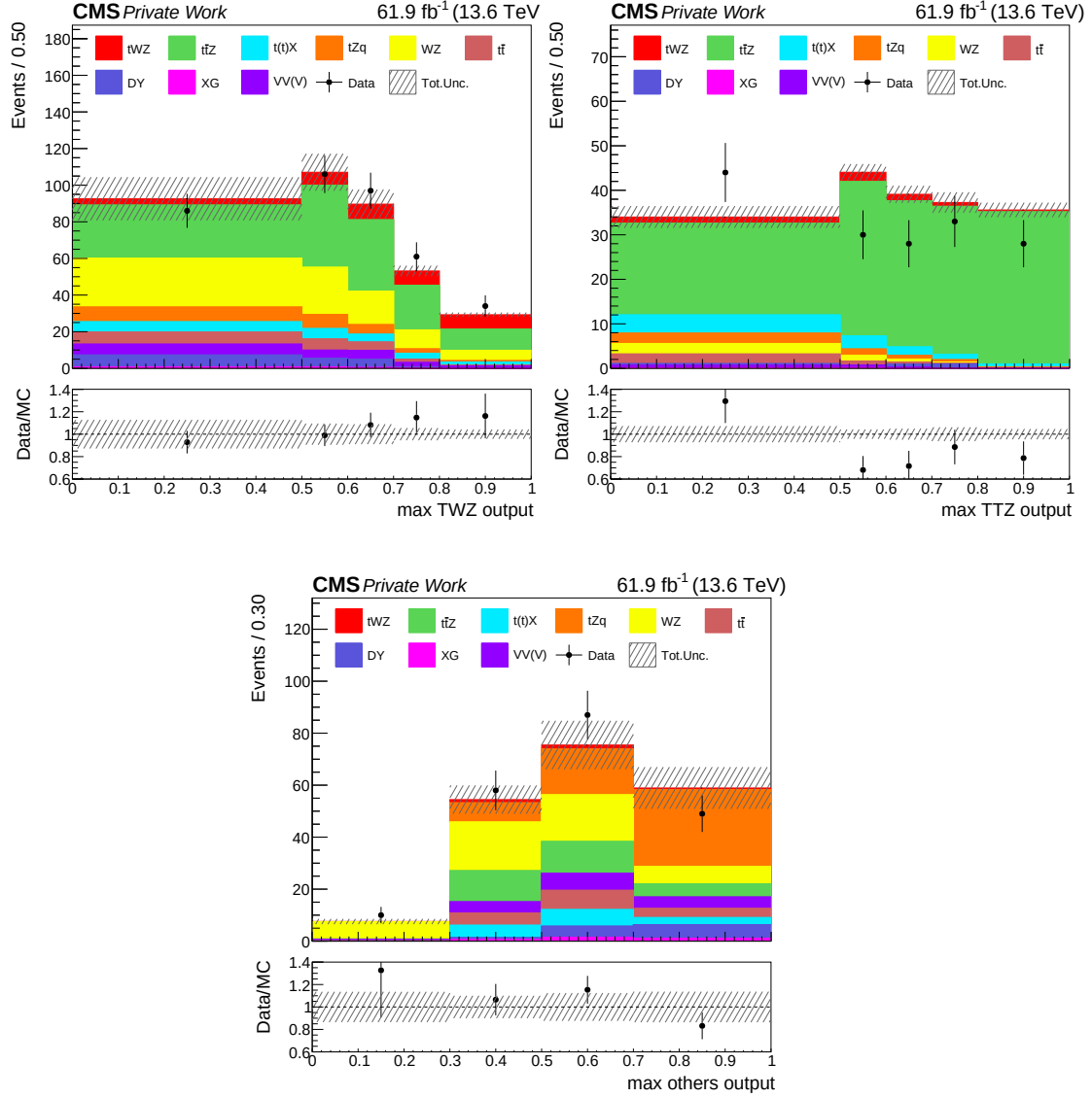
Figure 7.8: Maximum output scores of the three nodes in the 3 \ell SR for Run 3 data. The black markers represent the data, while the solid stacked histogram shows the MC predictions for the various background processes. The dashed band indicates the total uncertainty. The lower panel displays the ratio between data and simulation.
